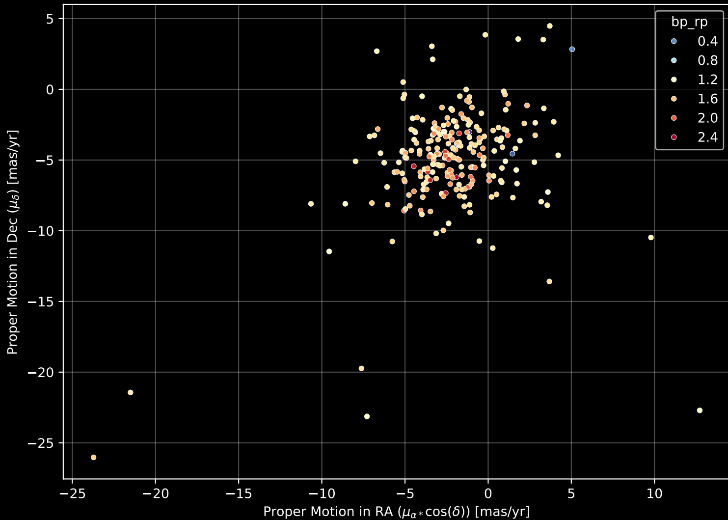
APOGEE DR17 Field: [340-10] Proper Motion Diagram (n= 244)
