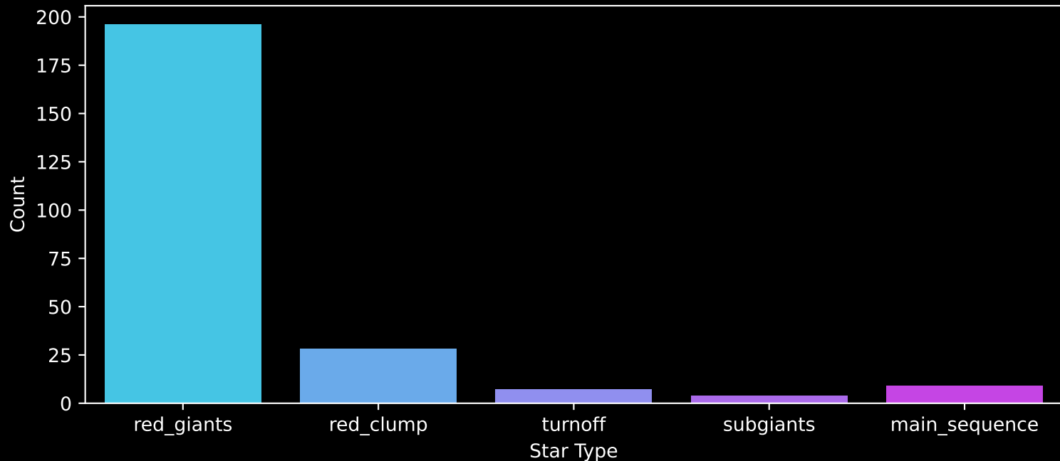
APOGEE DR17 Field: [340-10] Count plot of Star Type
