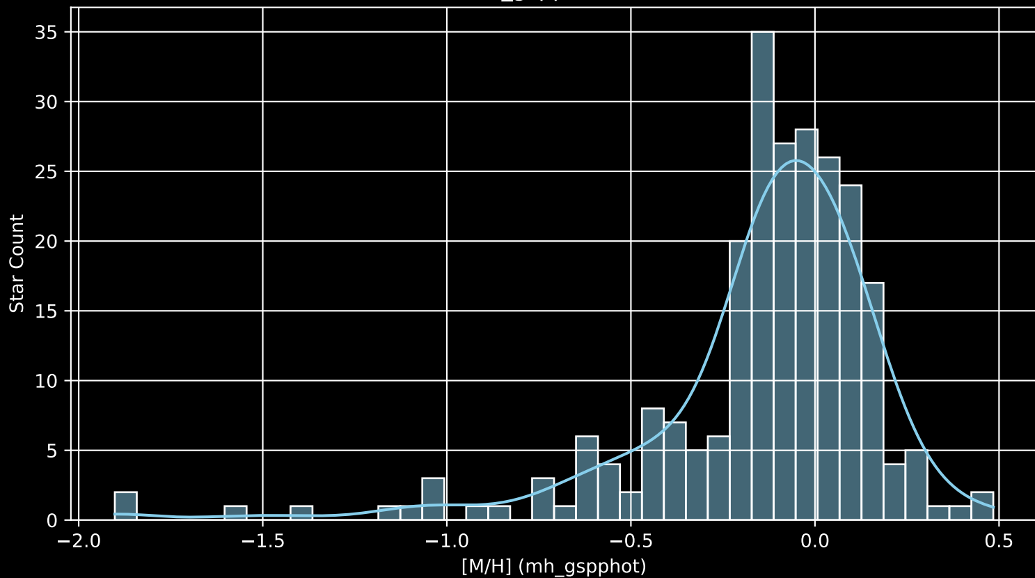
APOGEE DR17 Field: [340-10 [M/H] (mh_gspphot) (n= 243)
