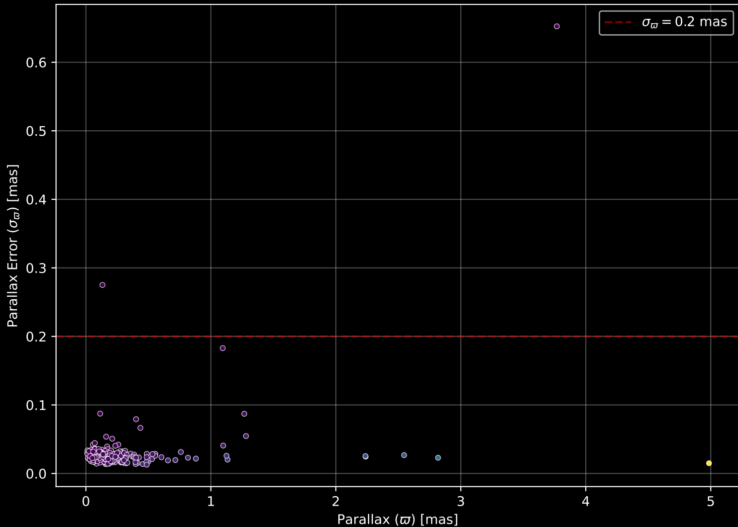
APOGEE DR17 Field: [340-10] Parallax Quality (n= 244)
