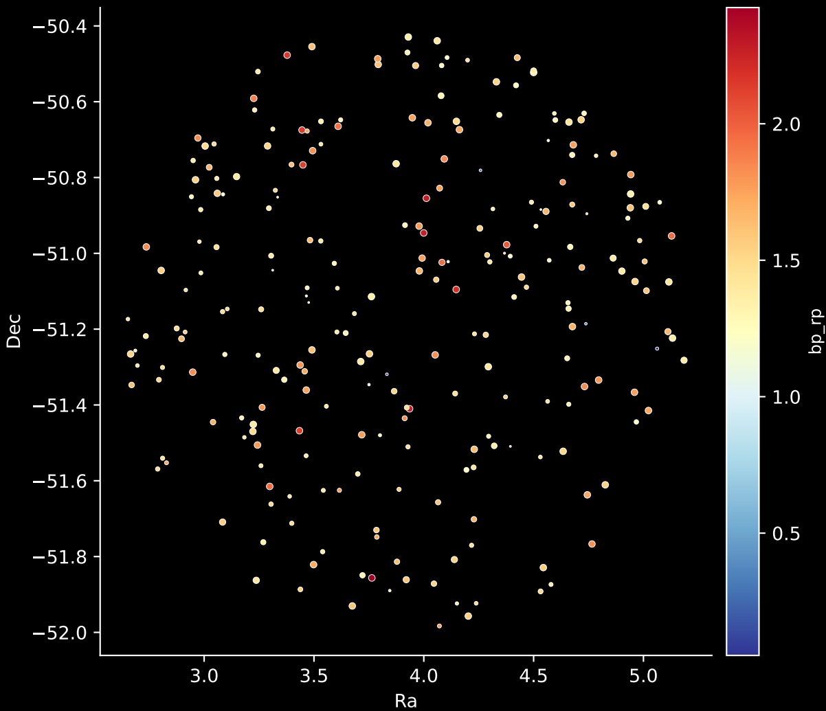
APOGEE DR17 Field: [340-10] Stars: 244
