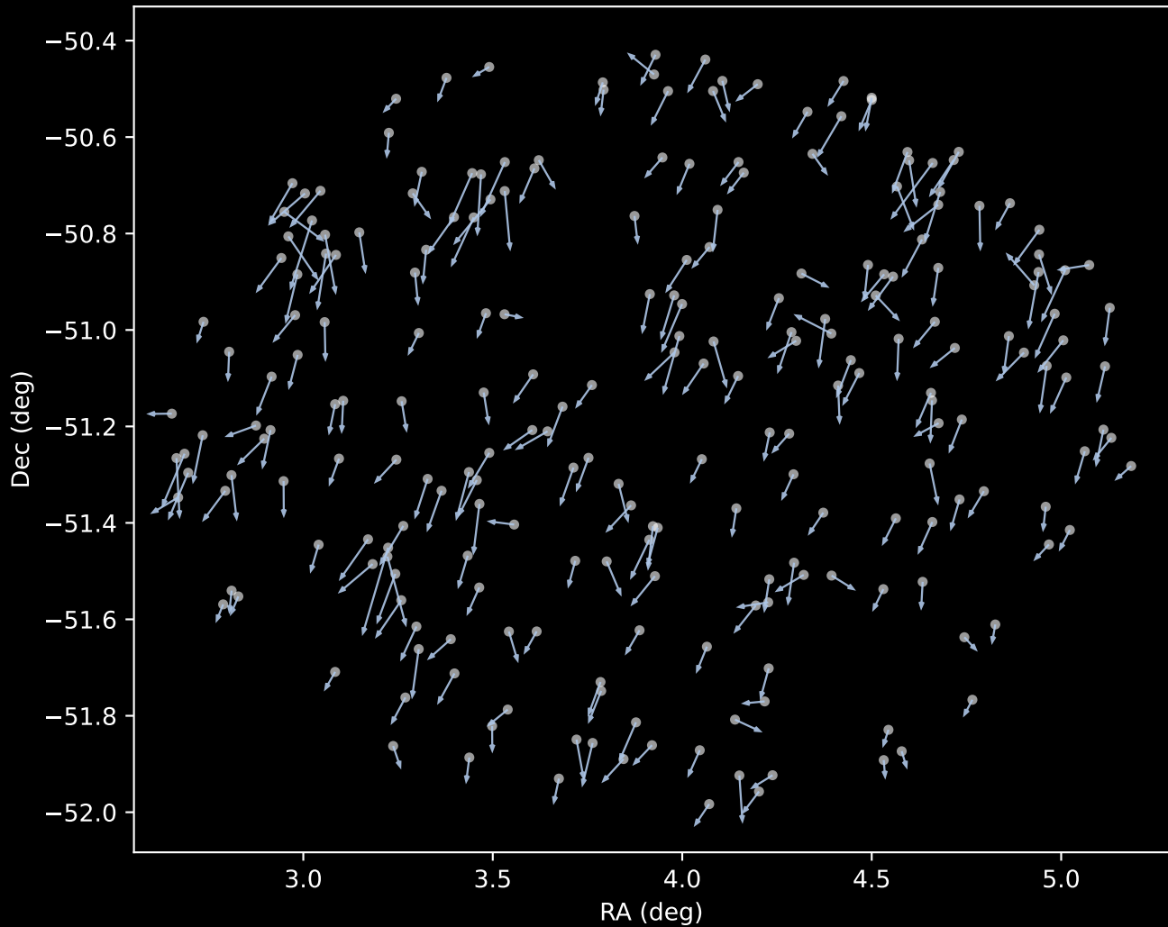
APOGEE DR17 Cluster 1 Proper Motion Vectors (n=230)
