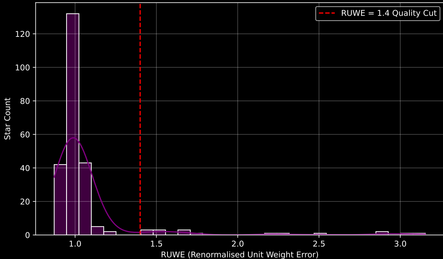
GAPOGEE DR17 Field [340-10] RUWE Distribution (n= 241)
